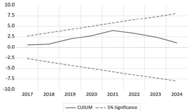
Hình 3. CUSUM stability plots of the ARDL(4, 3, 4, 3, 4)
