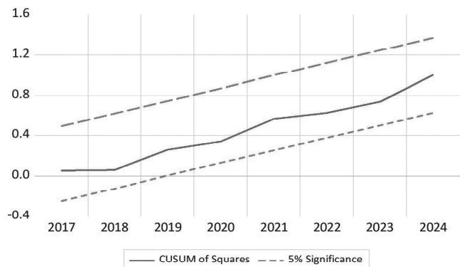
Hình 4. CUSUMQ stability plots of the ARDL(4, 3, 4, 3, 4)
